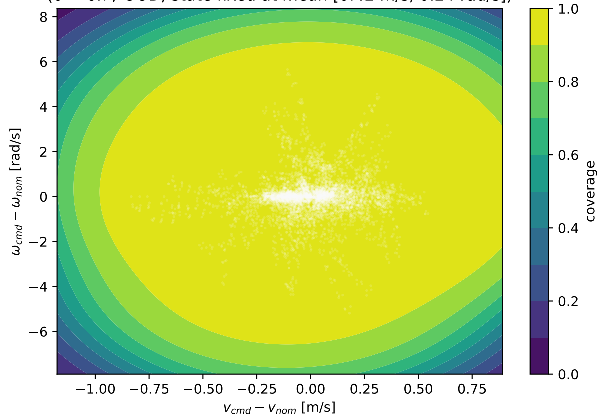
Residual coverage vs command offset (0 = off / OOD; state fixed at mean [0.42 m/s, 0.24 rad/s])
